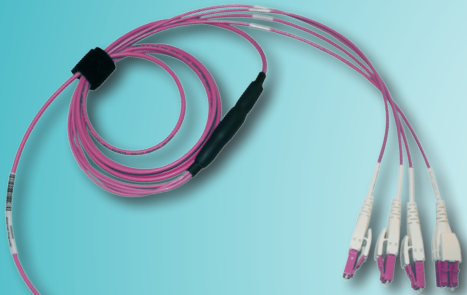
Erika Violet MTP® Cables 40G to 10G Fanout/Harness Cable
